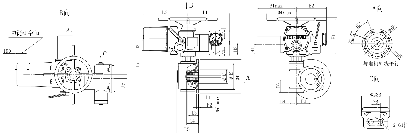
SMC-04~03. IN带HBC外形及连接尺寸
